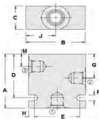
3 Way Housings
